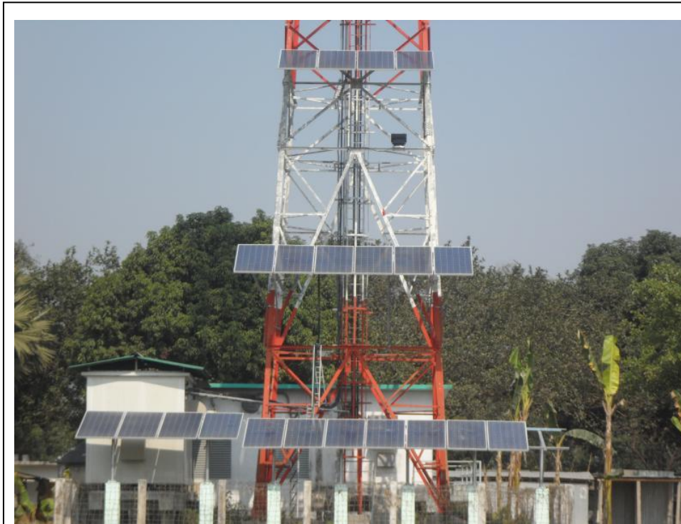
Solar Power for BTS Station installed by Allied Solar Energy Ltd. at Daridaha Bazar, Bogra
